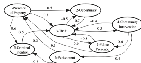
Figure 1. Example of an FCM about crime (source: Carvalho, 2013, p. 8)
